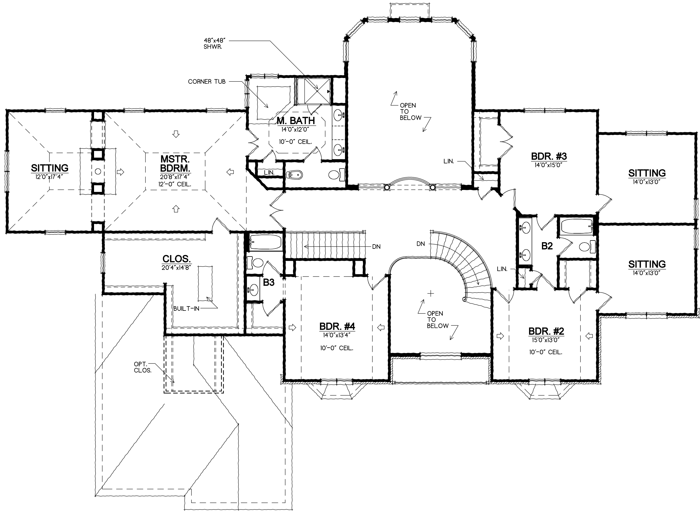
Optional 2nd Floor Scale: 1/8"=1'-0"
